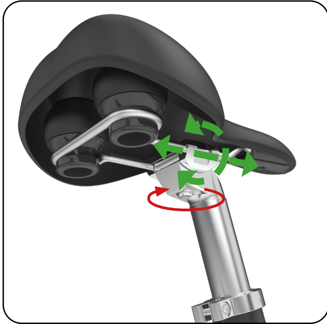
1 - Saddle
